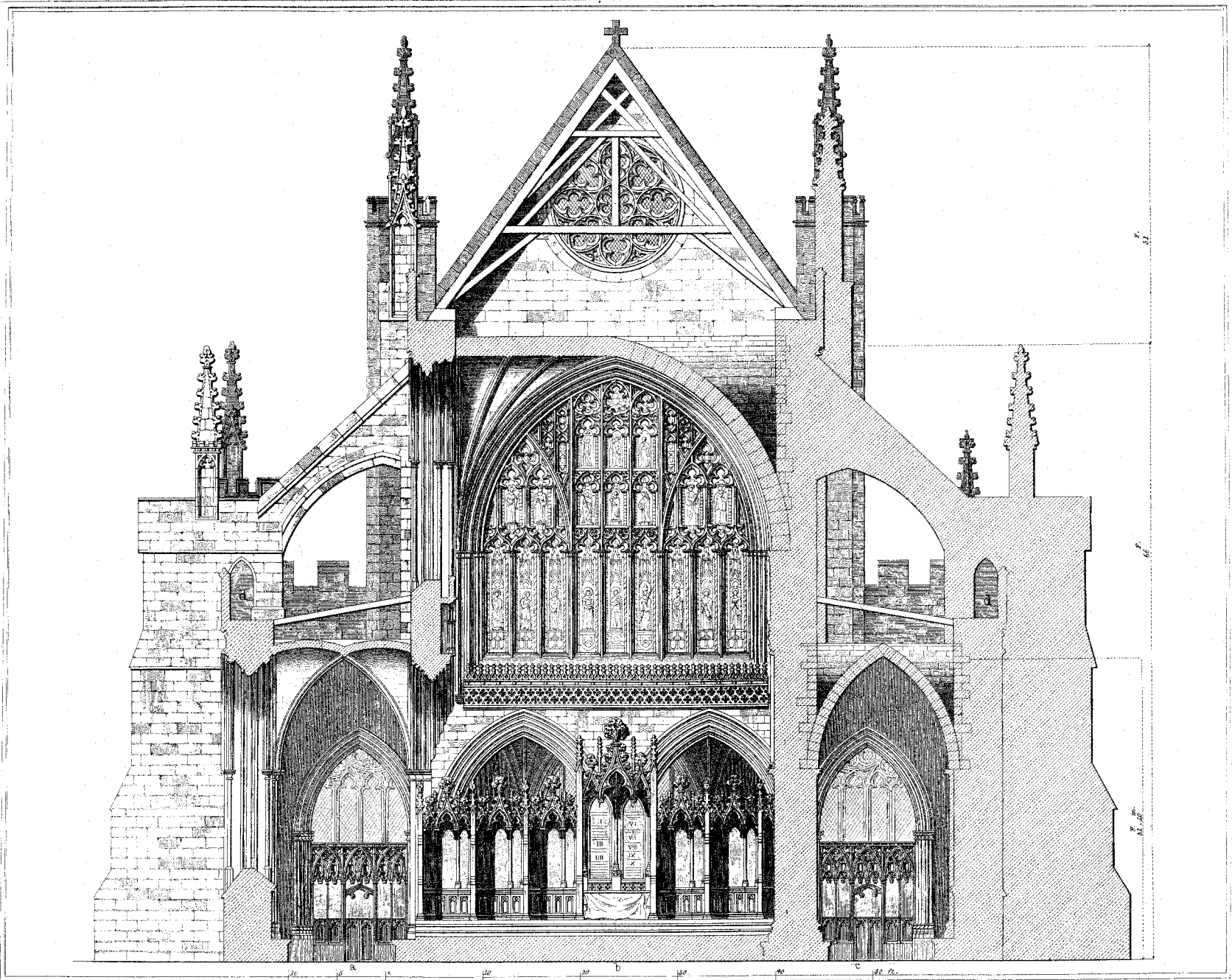
EXETER CATHEDRAL. SECTION OF EAST END, AT THE ALTAR.
